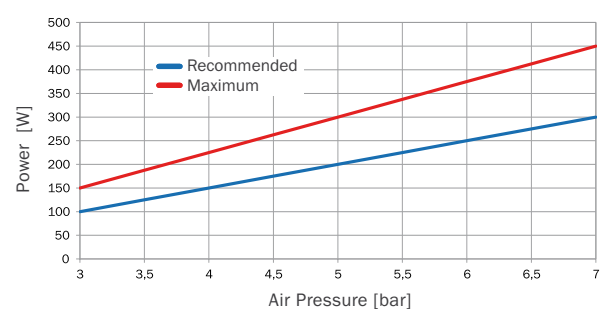
Power/Air Pressure
