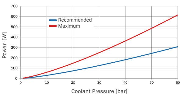
Power/Coolant Pressure
